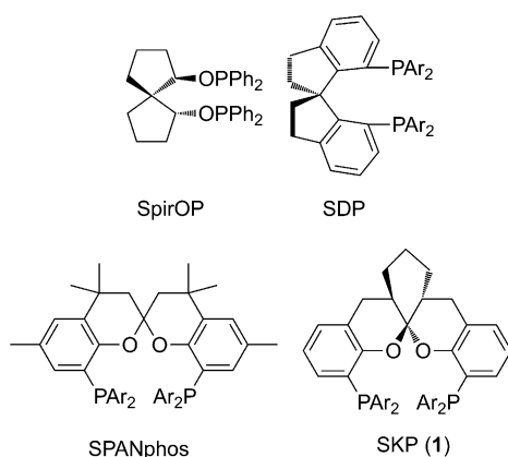
Scheme 1. Spiro-backbone-based bisphosphine ligands.
