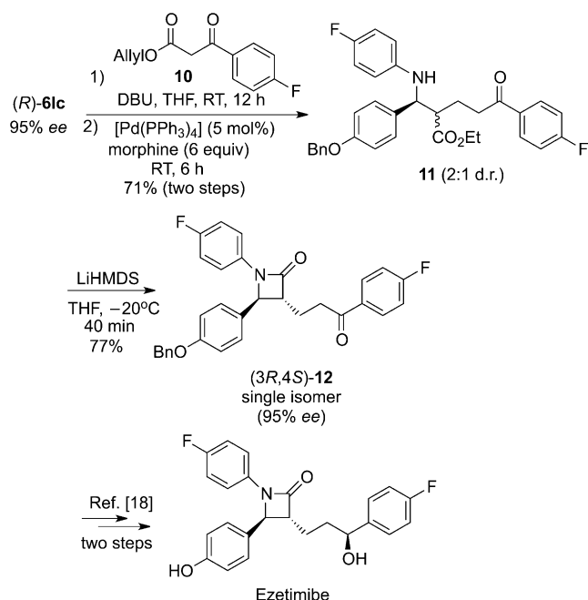
Scheme 4. Asymmetric synthesis of Ezetimibe using (R)-6lc as the key intermediate. Bn = benzyl, DBU = 1,8-diazabicyclo[5.4.0]undecene-7, HMDS = hexamethyldisilazide, THF = tetrahydrofuran.
