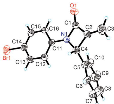
Figure 1. X-ray crystal structure ( S )- 8ad shown with thermal ellipsoids at 30% probability. [19]
