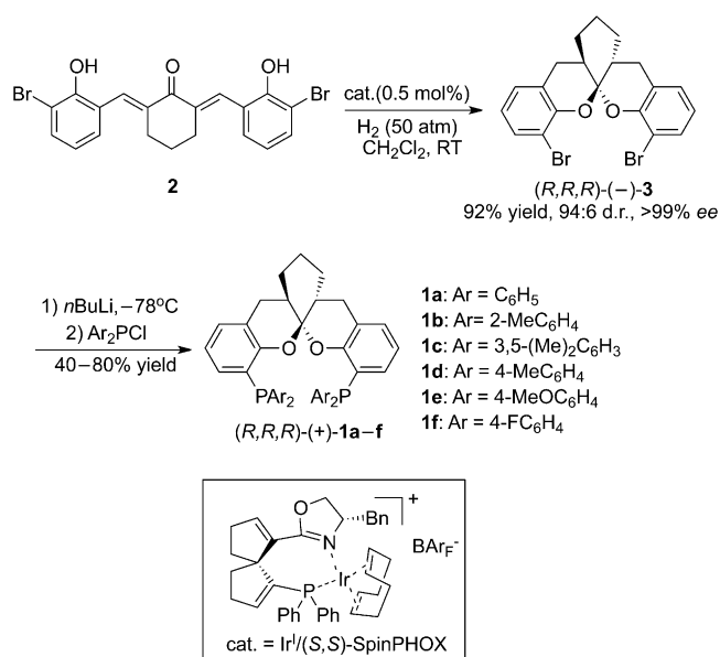
Scheme 2. Synthesis of enantiopure the spiro-2,2'-bis(chroman)-based bisphosphine ligands ( R,R,R )-1a–f.
