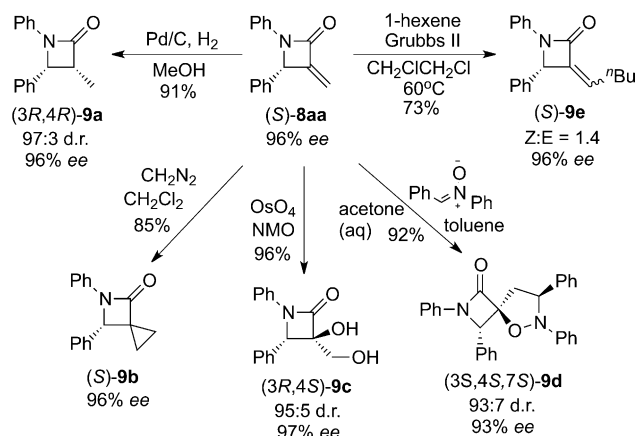
Scheme 3. Transformation of ( S )- 8aa into a variety of biologically interesting \beta -lactam derivatives ( 9a–e ). NMO = N -methylmorpholine N -oxide.
